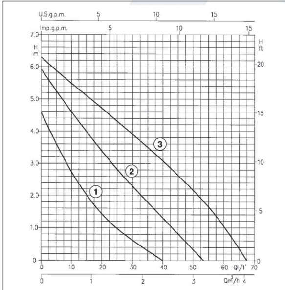
MR 63 range PERFORMANCE CURVES (according to ISO 9906 Attachment A)
