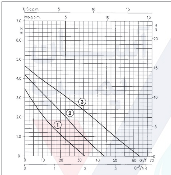
MR 63 range PERFORMANCE CURVES (according to ISO 9906 Attachment A)
